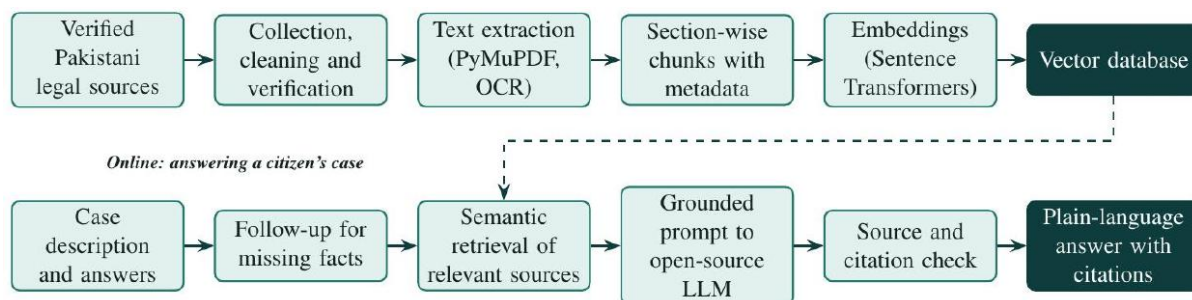
Figure 5: RAG pipeline — offline knowledge base preparation and online answering
